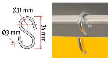
Gancio a "S" metallico porta banner. Metal "S" shaped hook for aisle sign fixtures.
